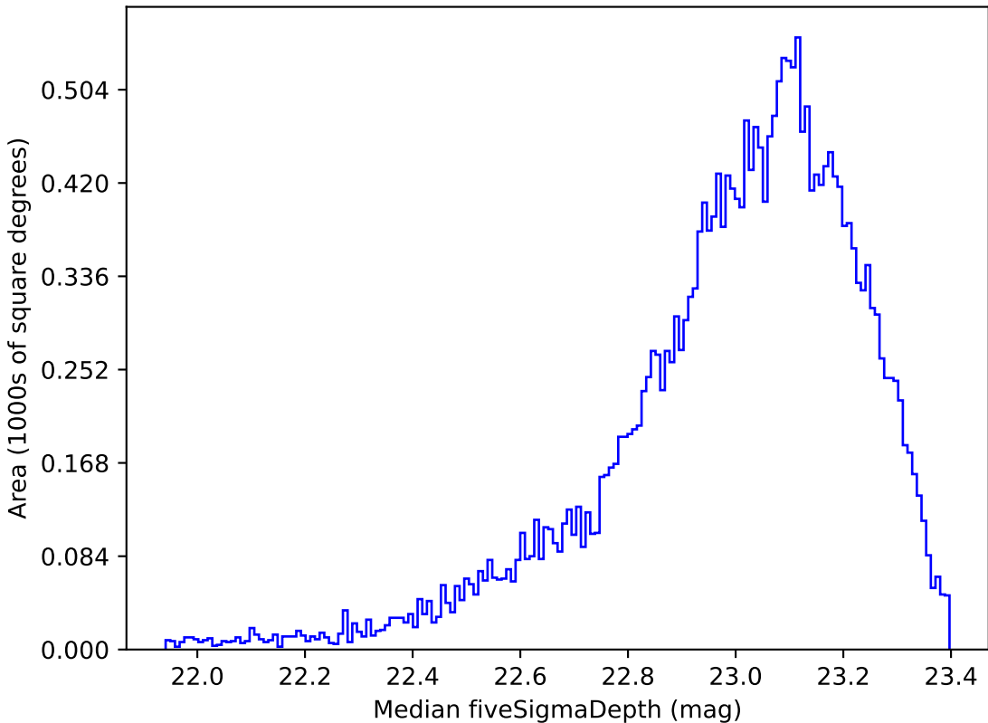
noroll_mjdp365_v3.4_10yrs Yr 1 z band: Median fiveSigmaDepth
