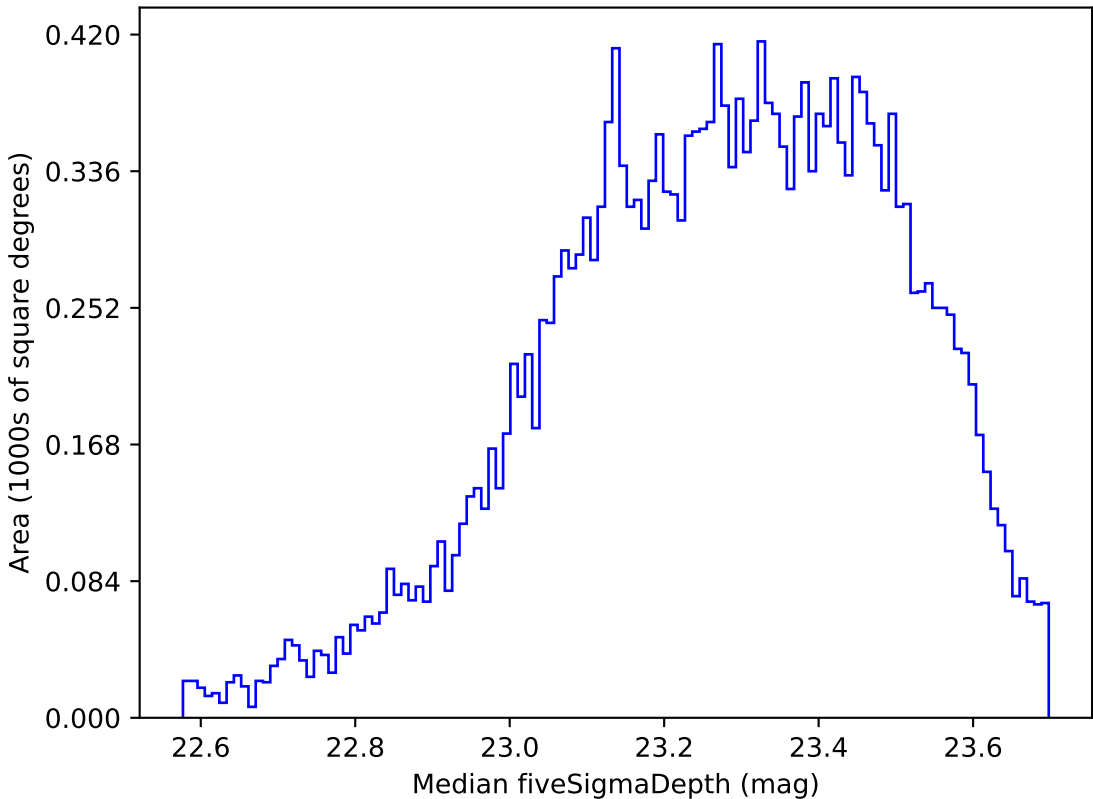
noroll_mjdp365_v3.4_10yrs Yr 1 u band: Median fiveSigmaDepth
