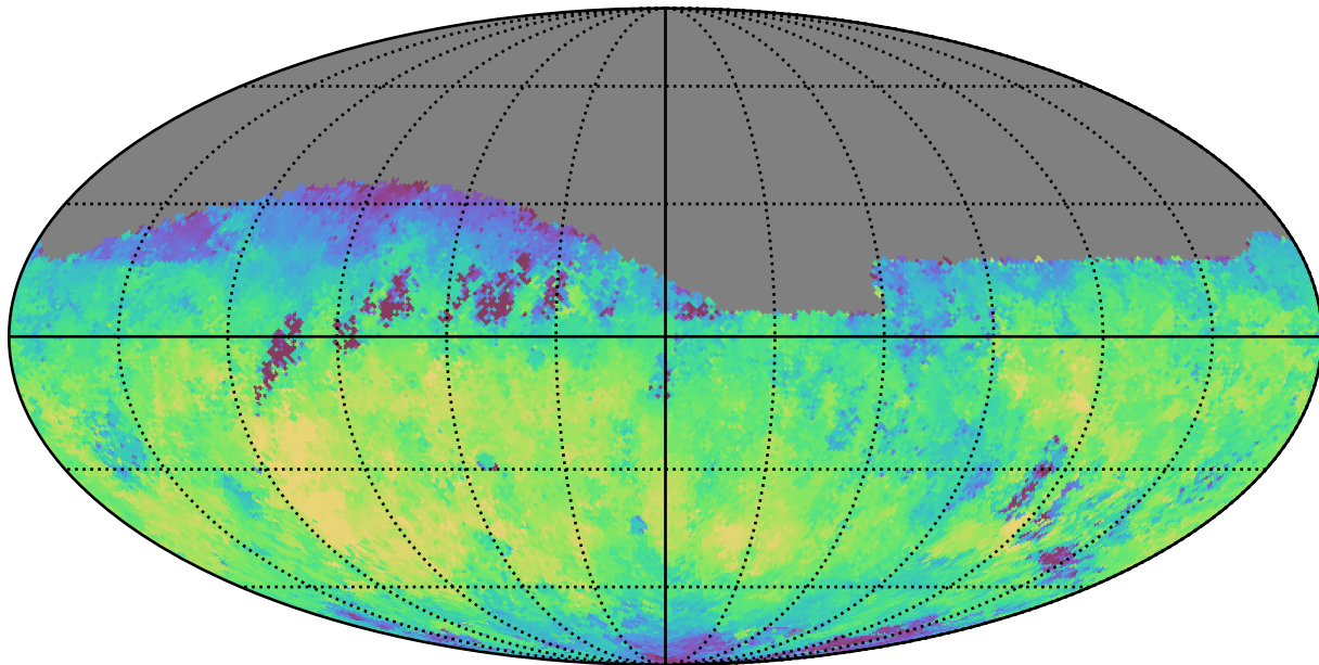
noroll_mjdp365_v3.4_10yrs Yr 1 r band: Median fiveSigmaDepth
