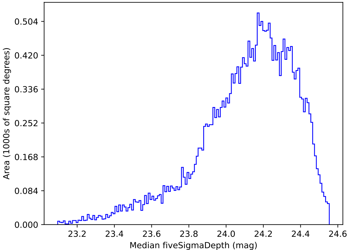
noroll_mjdp365_v3.4_10yrs Yr 1 r band: Median fiveSigmaDepth
