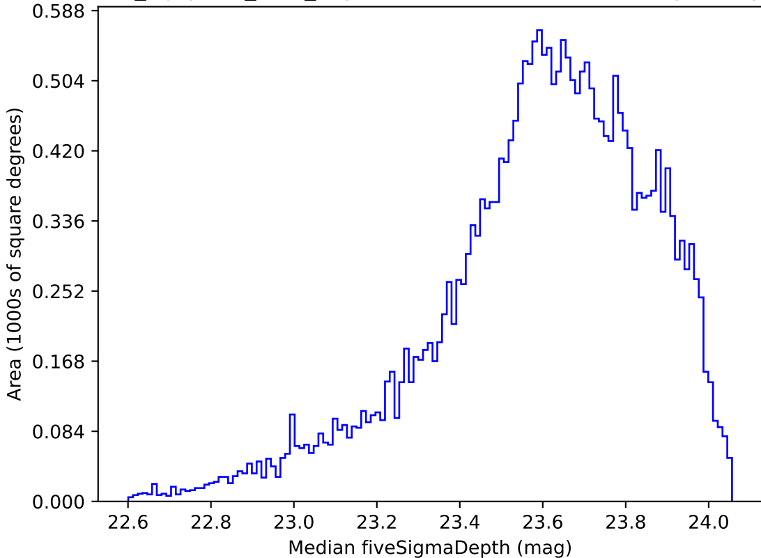
noroll_mjdp365_v3.4_10yrs Yr 1 i band: Median fiveSigmaDepth
