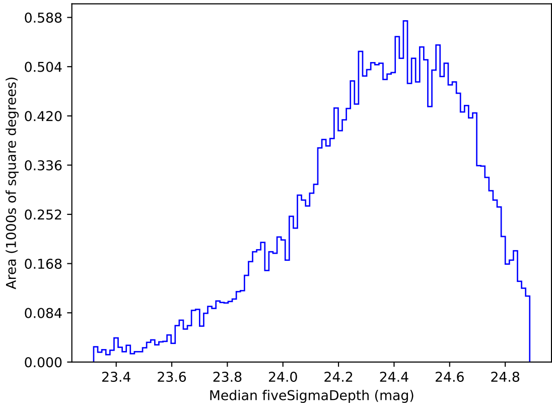
noroll_mjdp365_v3.4_10yrs Yr 1 g band: Median fiveSigmaDepth
