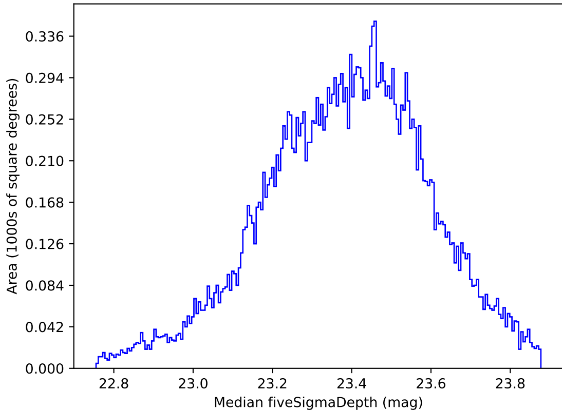
noroll_mjdp365_v3.4_10yrs Yr 1 all bands: Median fiveSigmaDepth
