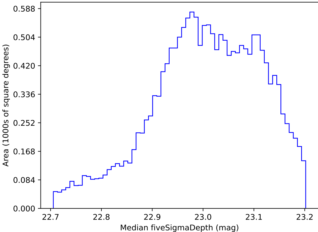
noroll_mjdp365_v3.4_10yrs WFD z band: Median fiveSigmaDepth
