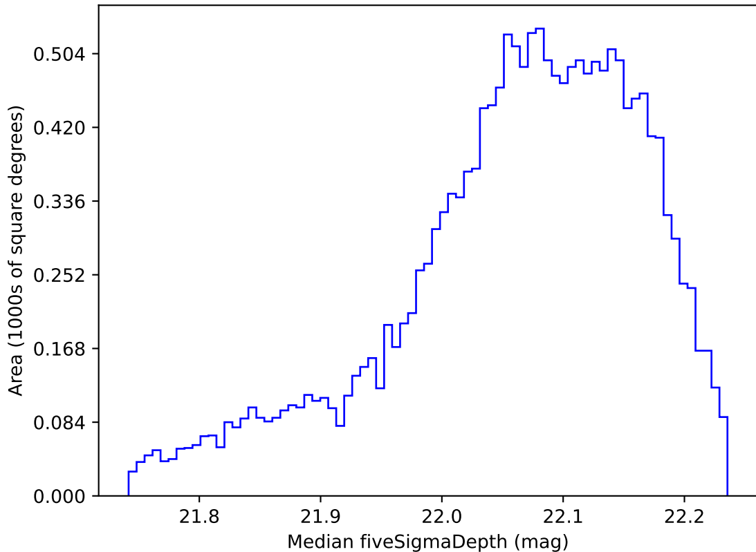
noroll_mjdp365_v3.4_10yrs WFD y band: Median fiveSigmaDepth
