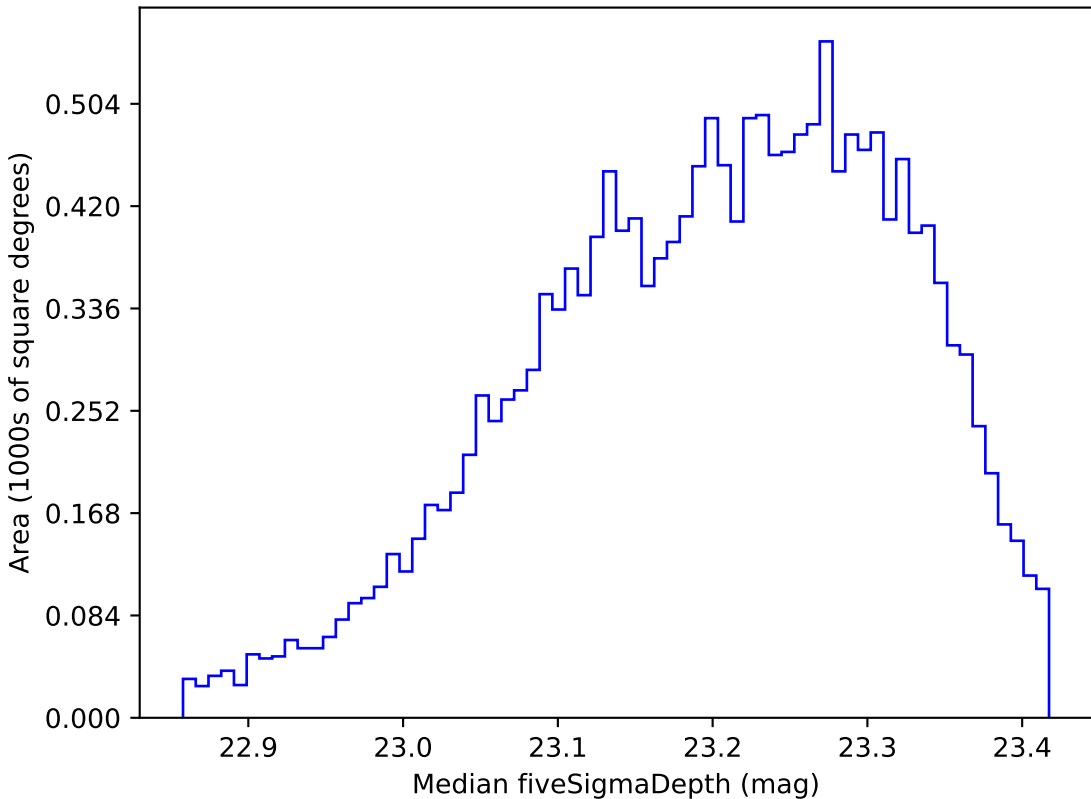
noroll_mjdp365_v3.4_10yrs WFD u band: Median fiveSigmaDepth
