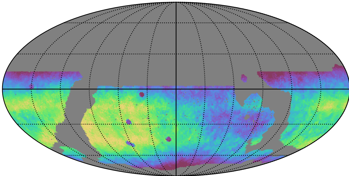
noroll_mjdp365_v3.4_10yrs WFD r band: Median fiveSigmaDepth
