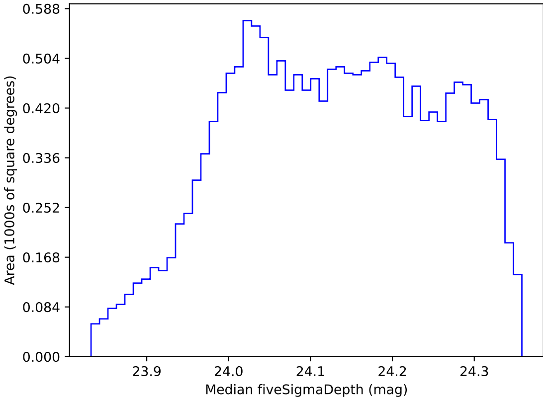
noroll_mjdp365_v3.4_10yrs WFD r band: Median fiveSigmaDepth
