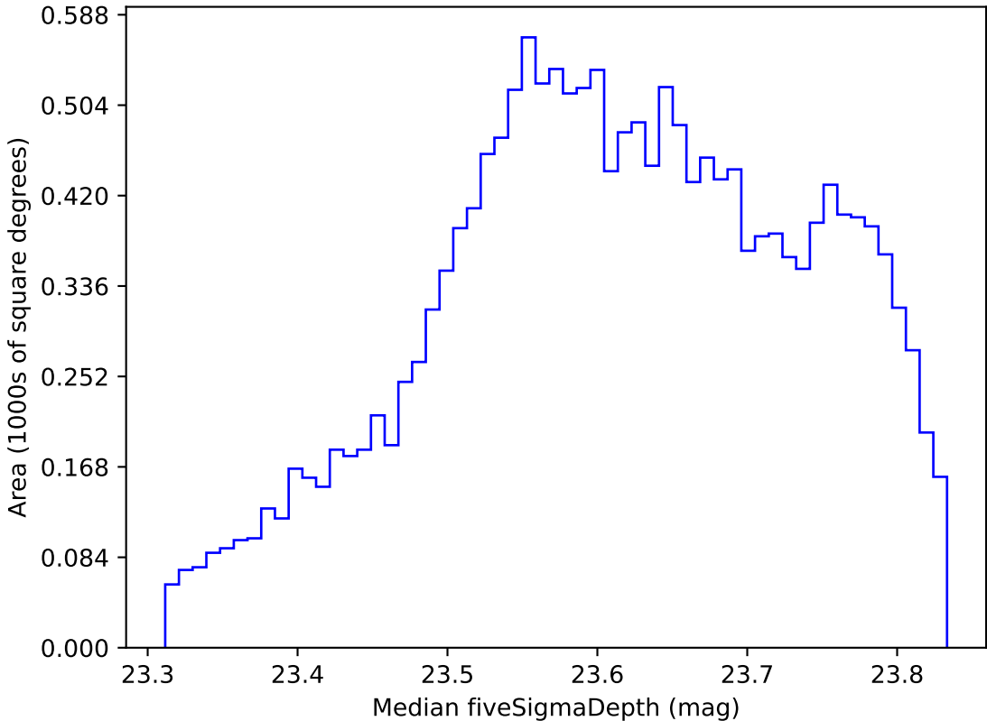
noroll_mjdp365_v3.4_10yrs WFD i band: Median fiveSigmaDepth
