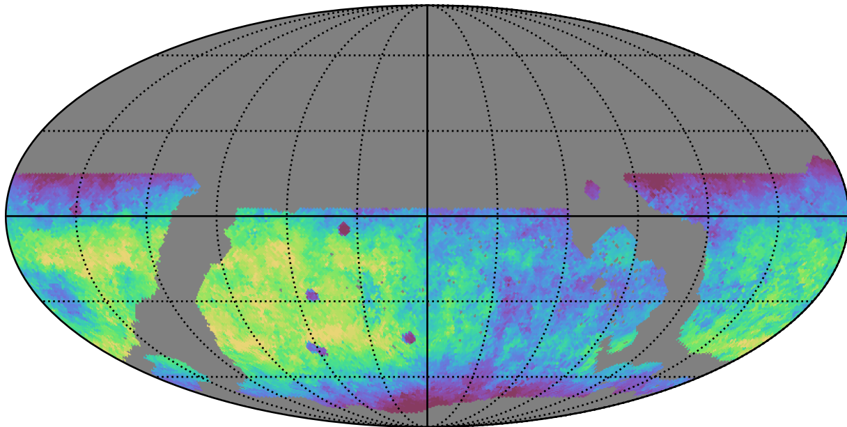
noroll_mjdp365_v3.4_10yrs WFD g band: Median fiveSigmaDepth
