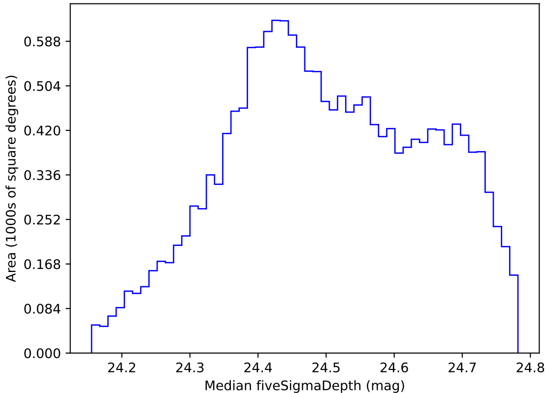
noroll_mjdp365_v3.4_10yrs WFD g band: Median fiveSigmaDepth
