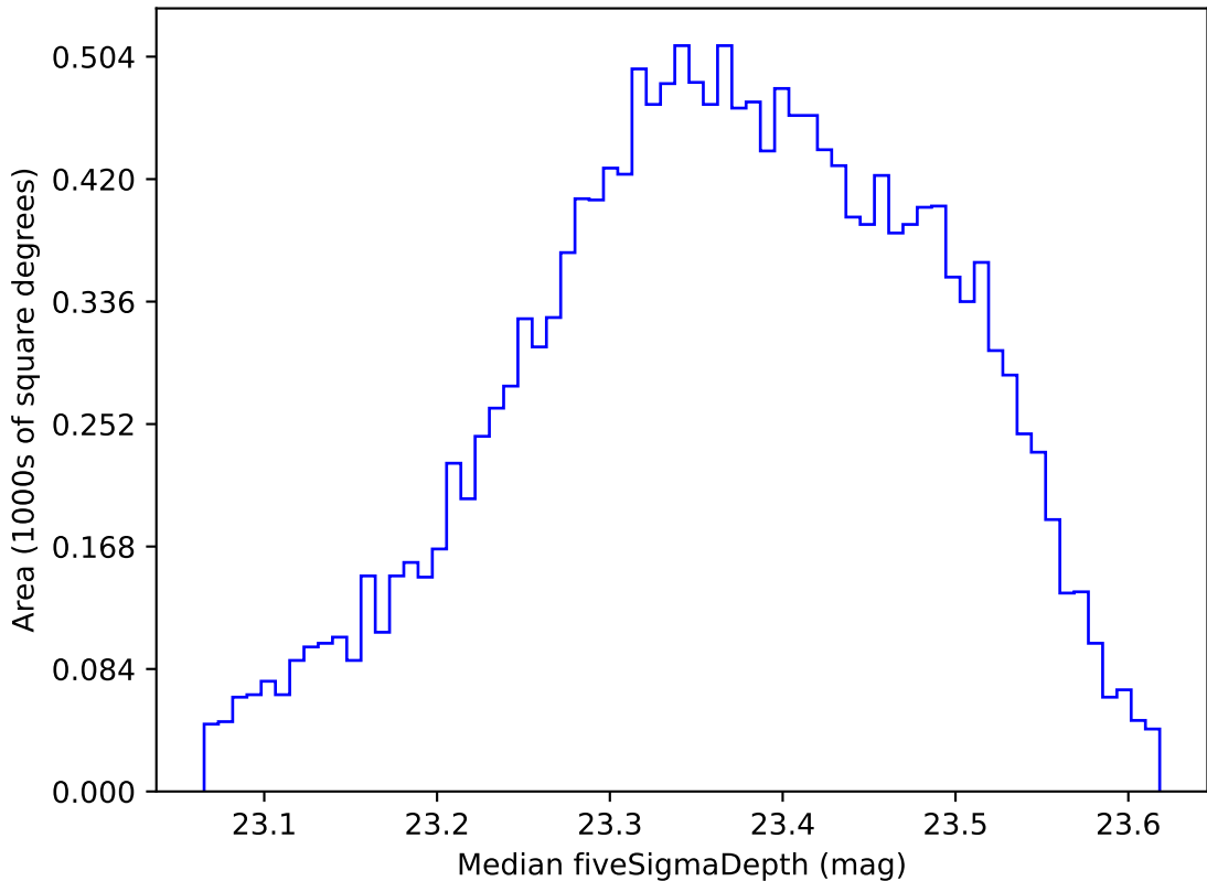
noroll_mjdp365_v3.4_10yrs WFD all bands: Median fiveSigmaDepth
