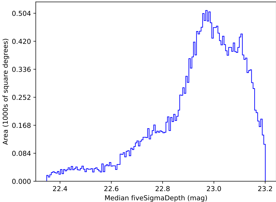
noroll_mjdp365_v3.4_10yrs All sky z band: Median fiveSigmaDepth
