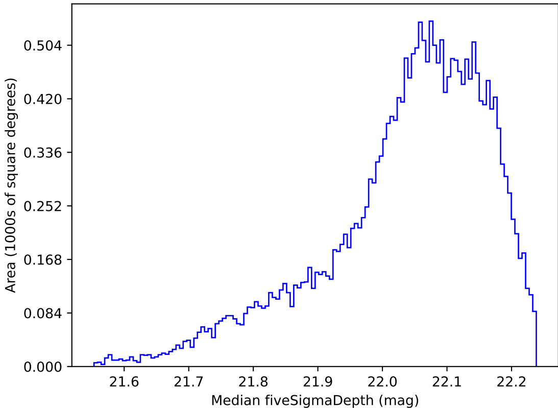
noroll_mjdp365_v3.4_10yrs All sky y band: Median fiveSigmaDepth
