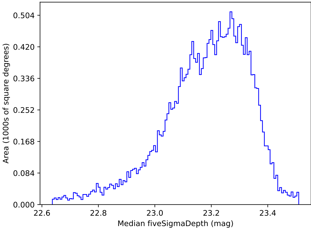
noroll_mjdp365_v3.4_10yrs All sky u band: Median fiveSigmaDepth
