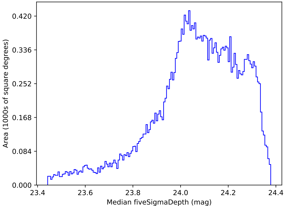
noroll_mjdp365_v3.4_10yrs All sky r band: Median fiveSigmaDepth
