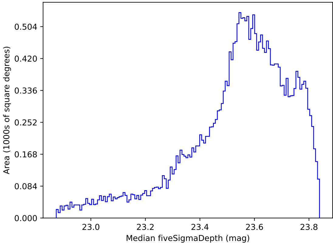
noroll_mjdp365_v3.4_10yrs All sky i band: Median fiveSigmaDepth
