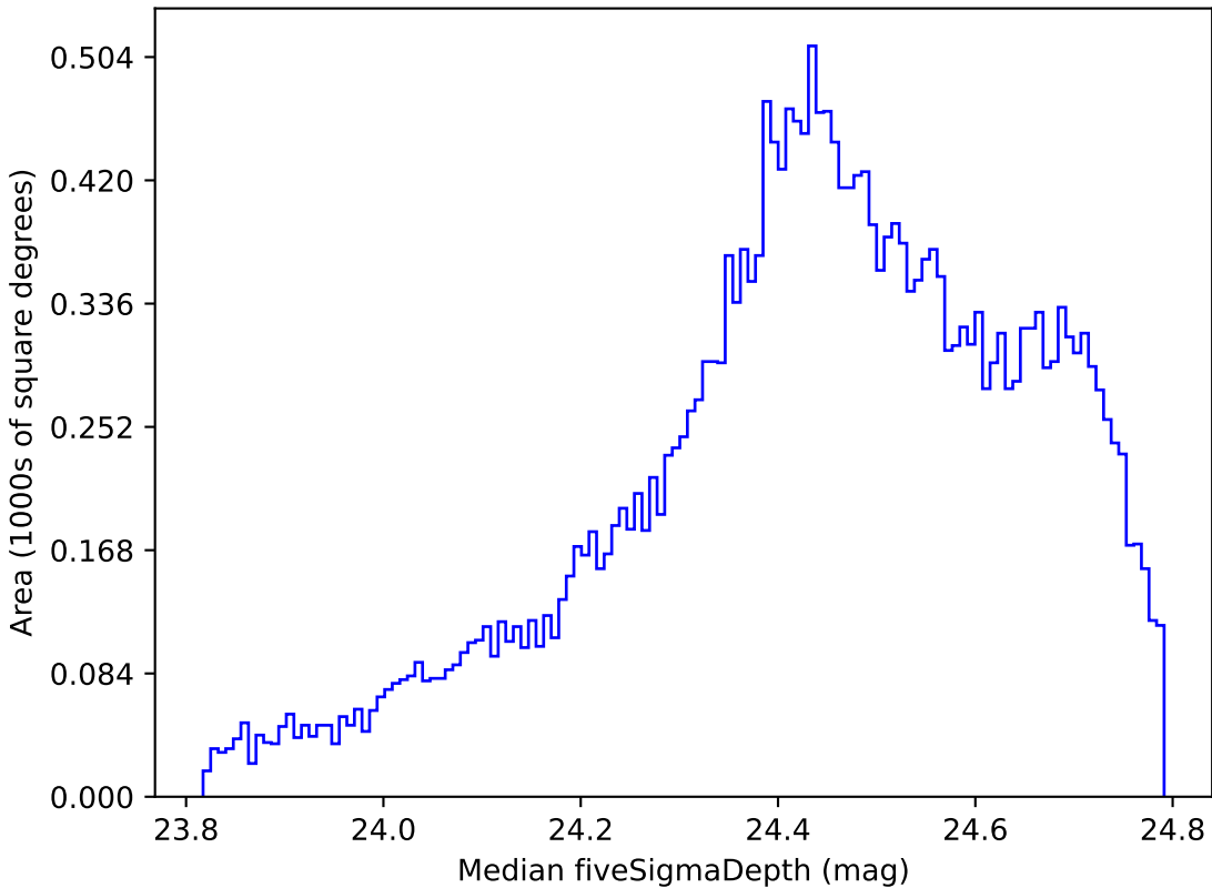
noroll_mjdp365_v3.4_10yrs All sky g band: Median fiveSigmaDepth
