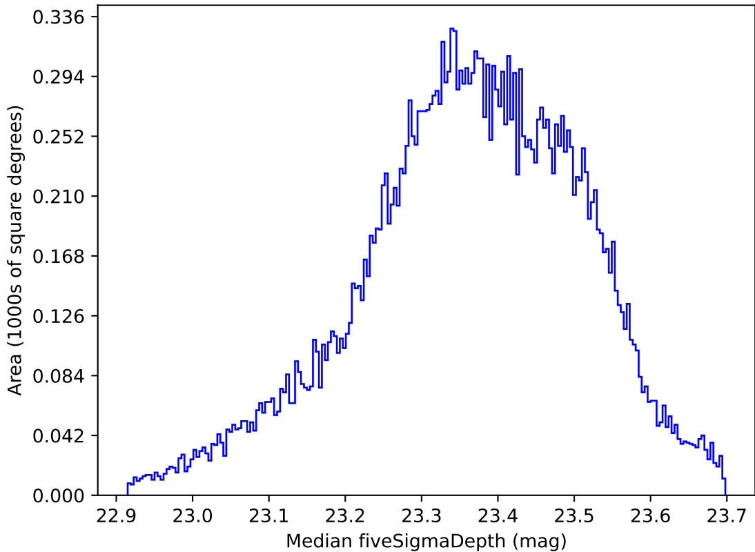
noroll_mjdp365_v3.4_10yrs All sky all bands: Median fiveSigmaDepth
