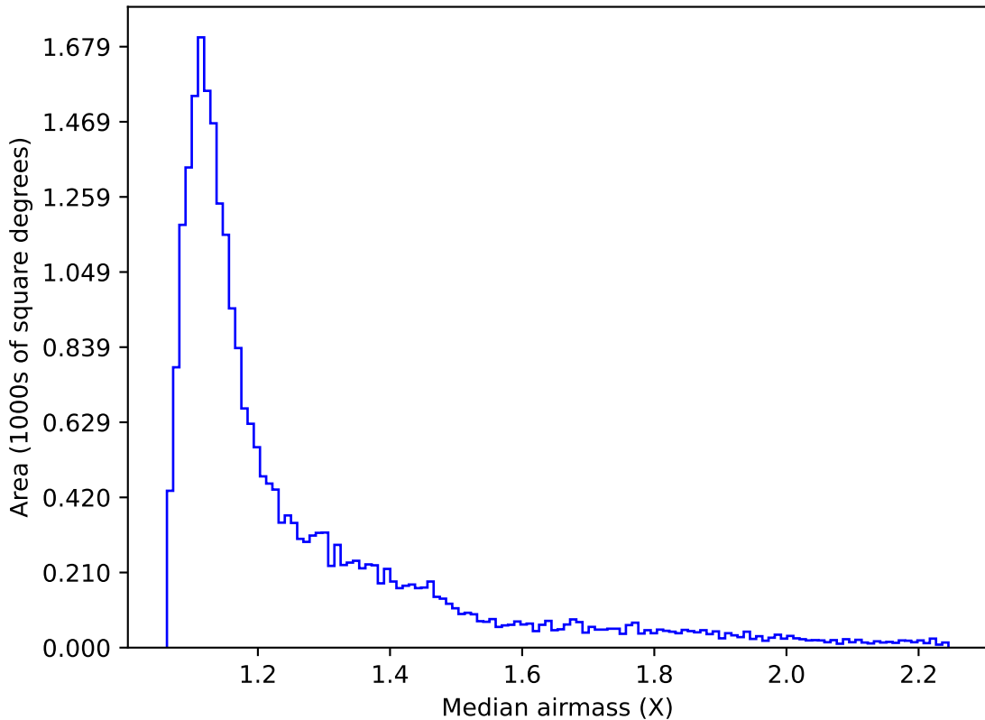
noroll_mjdp365_v3.4_10yrs Yr 1 z band: Median airmass
