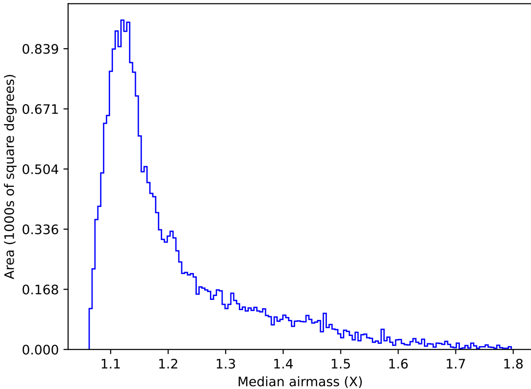
noroll_mjdp365_v3.4_10yrs Yr 1 y band: Median airmass
