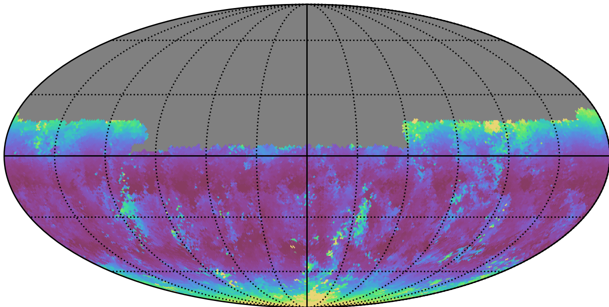
noroll_mjdp365_v3.4_10yrs Yr 1 u band: Median airmass
