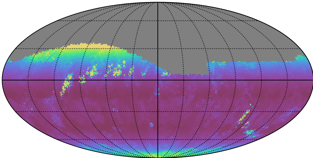
noroll_mjdp365_v3.4_10yrs Yr 1 r band: Median airmass
