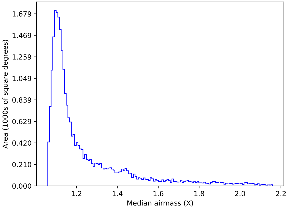
noroll_mjdp365_v3.4_10yrs Yr 1 i band: Median airmass
