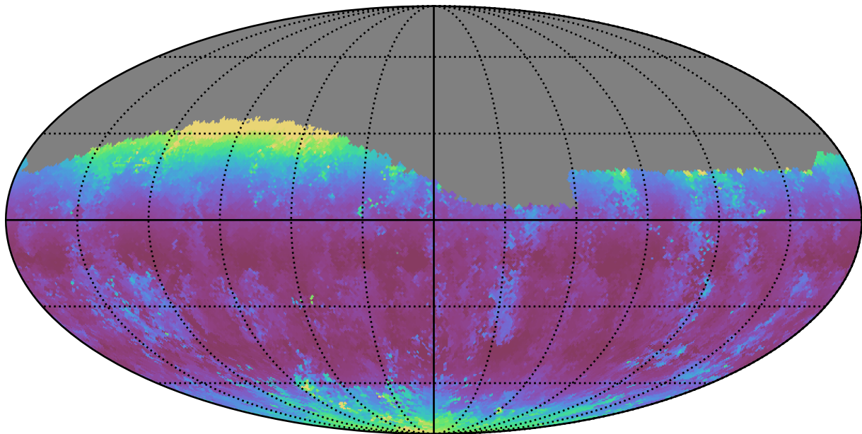
noroll_mjdp365_v3.4_10yrs Yr 1 g band: Median airmass
