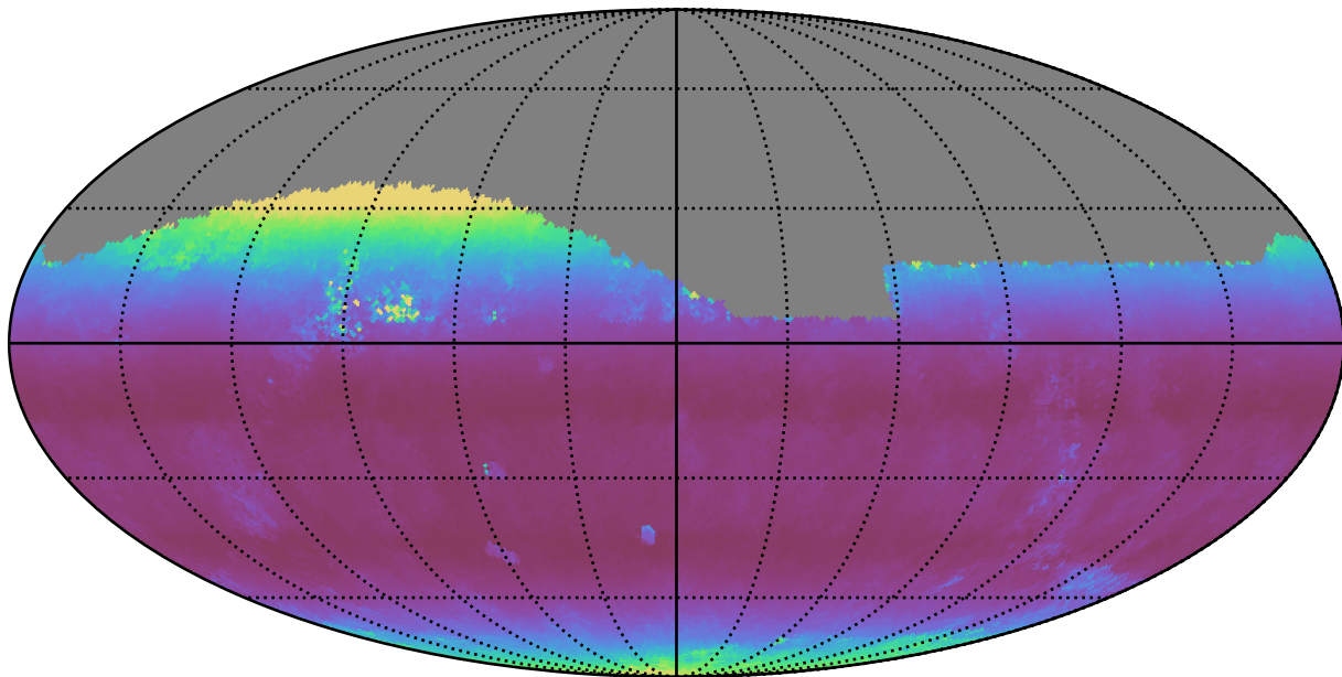
noroll_mjdp365_v3.4_10yrs Yr 1 all bands: Median airmass
