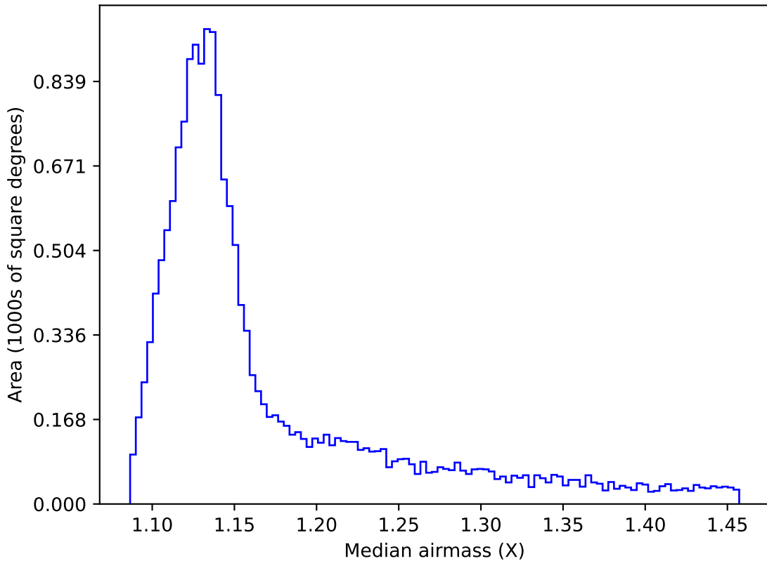
noroll_mjdp365_v3.4_10yrs WFD y band: Median airmass
