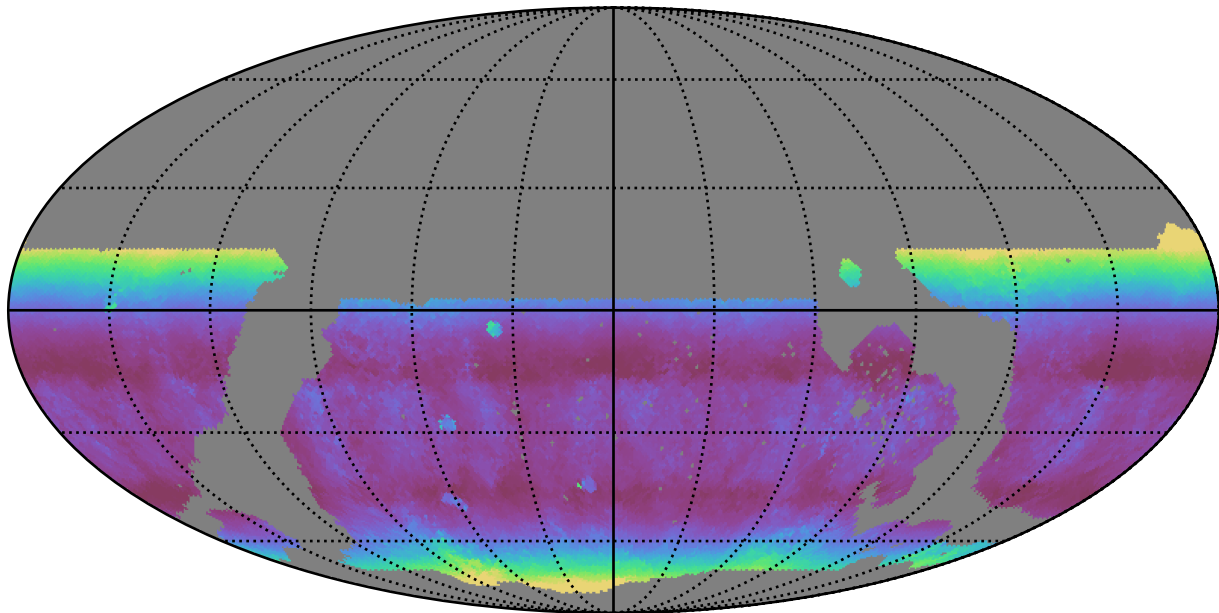
noroll_mjdp365_v3.4_10yrs WFD u band: Median airmass
