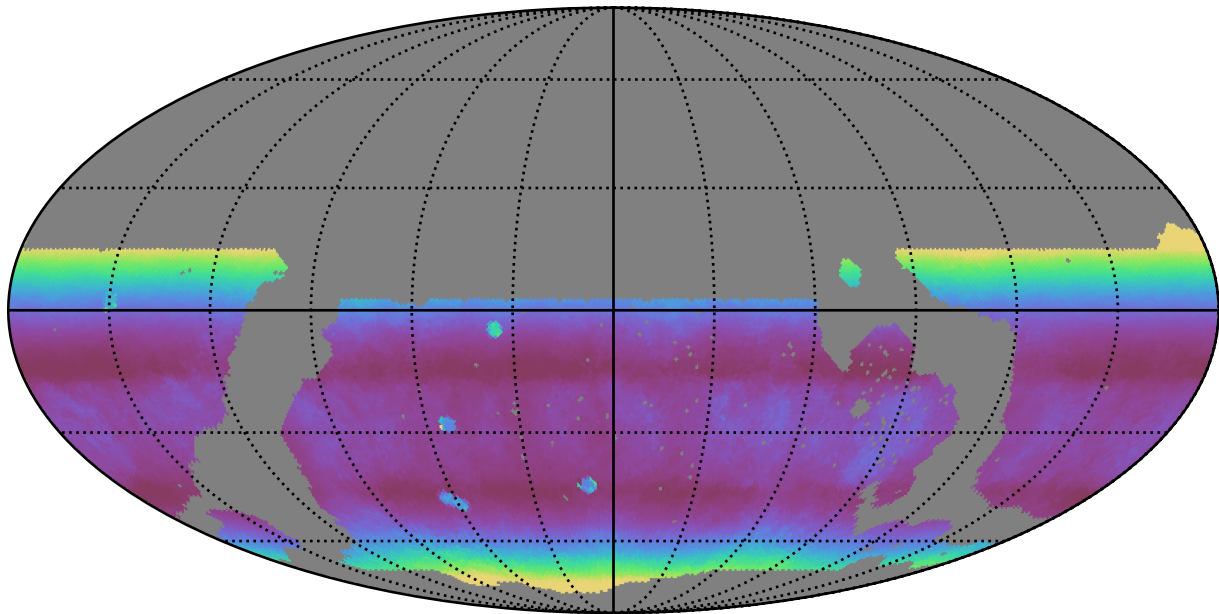
noroll_mjdp365_v3.4_10yrs WFD r band: Median airmass
