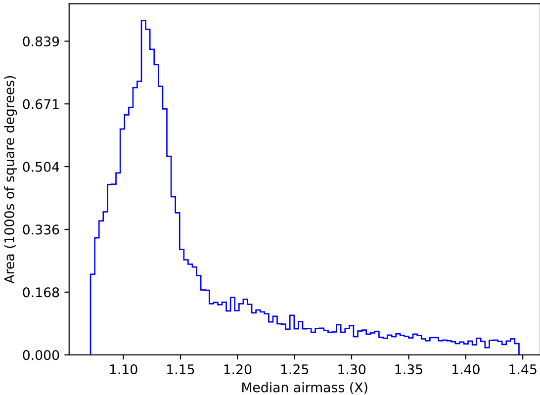
noroll_mjdp365_v3.4_10yrs WFD r band: Median airmass
