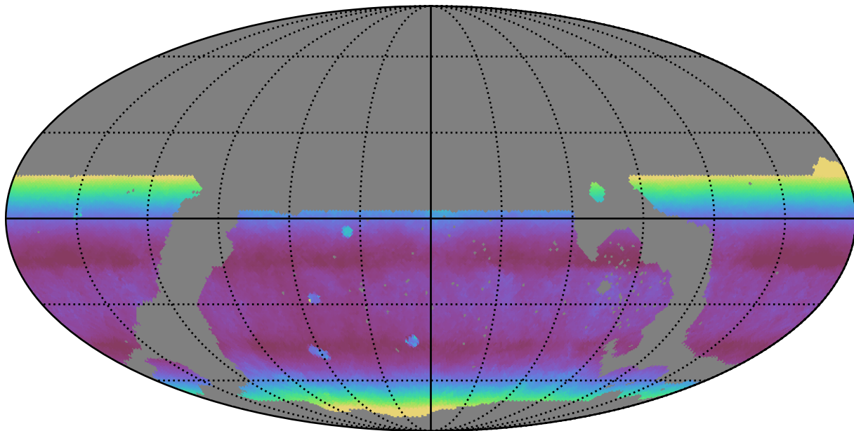
noroll_mjdp365_v3.4_10yrs WFD i band: Median airmass
