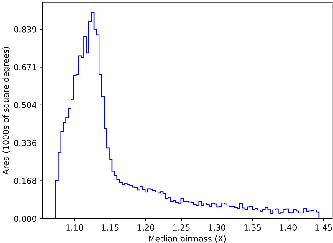
noroll_mjdp365_v3.4_10yrs WFD i band: Median airmass
