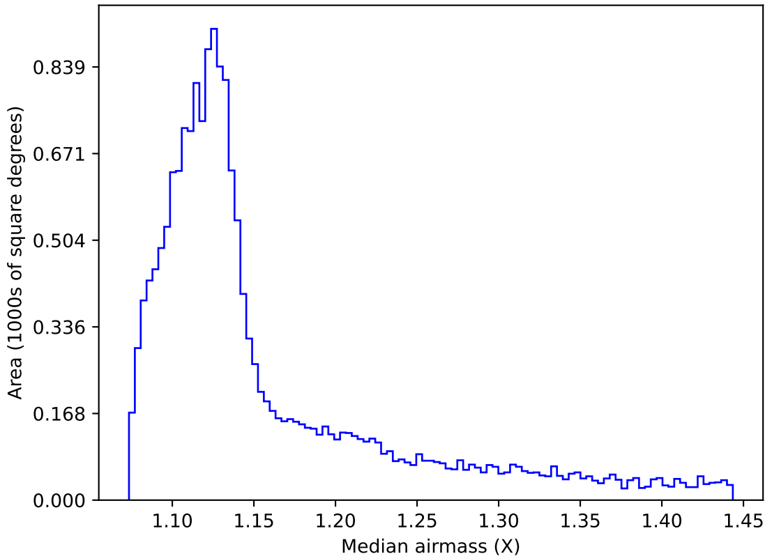
noroll_mjdp365_v3.4_10yrs WFD i band: Median airmass
