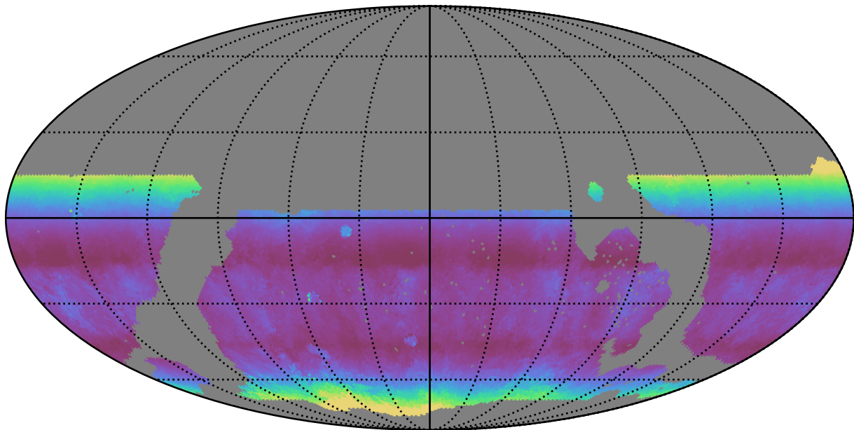
noroll_mjdp365_v3.4_10yrs WFD g band: Median airmass
