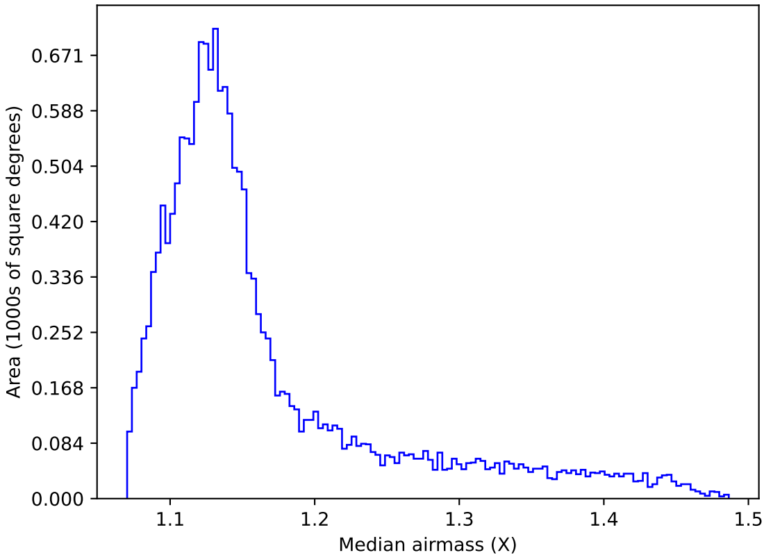
noroll_mjdp365_v3.4_10yrs WFD g band: Median airmass
