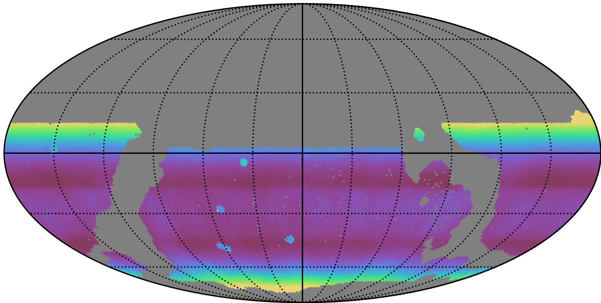
noroll_mjdp365_v3.4_10yrs WFD all bands: Median airmass
