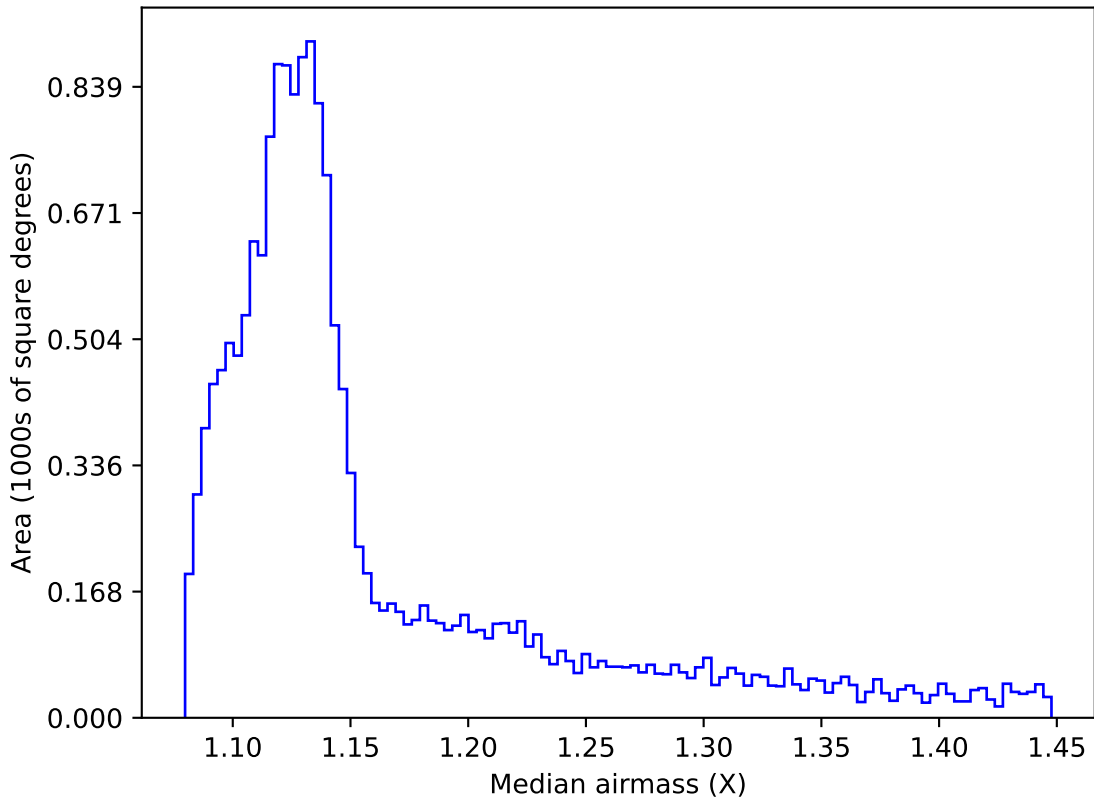
noroll_mjdp365_v3.4_10yrs WFD all bands: Median airmass
