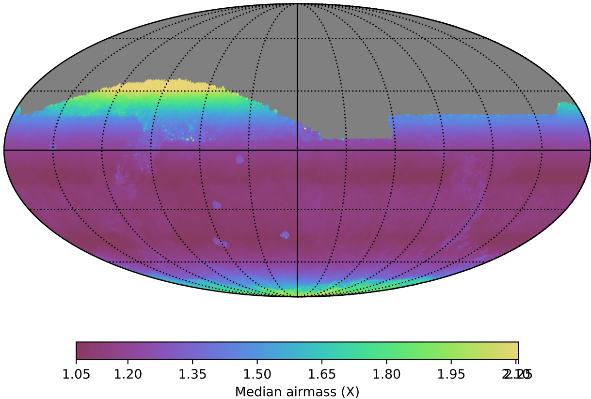
noroll_mjdp365_v3.4_10yrs All sky z band: Median airmass
