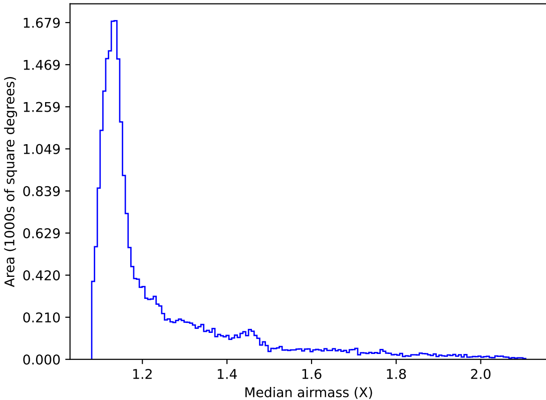
noroll_mjdp365_v3.4_10yrs All sky z band: Median airmass
