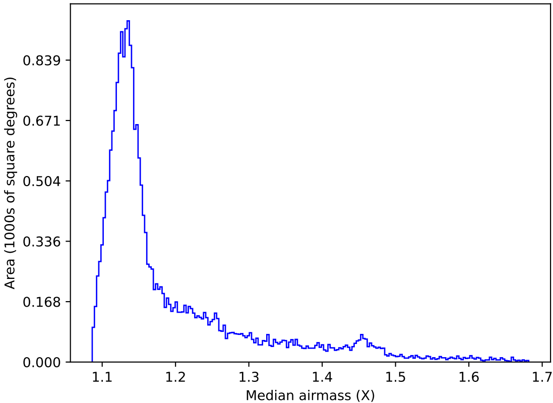
noroll_mjdp365_v3.4_10yrs All sky y band: Median airmass
