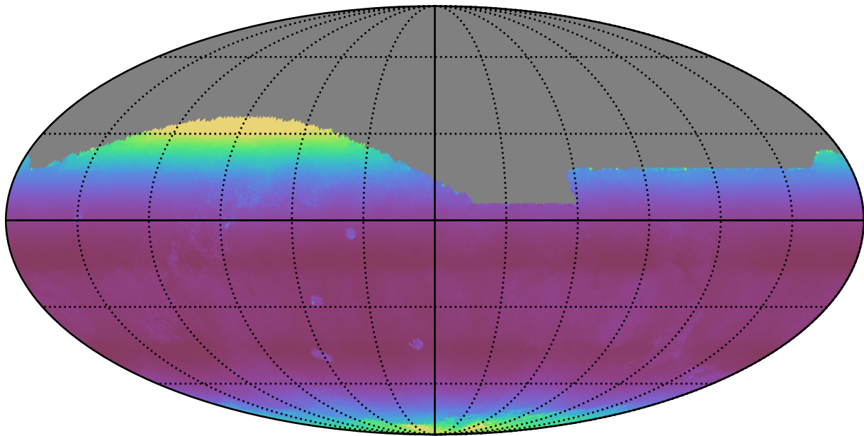
noroll_mjdp365_v3.4_10yrs All sky r band: Median airmass
