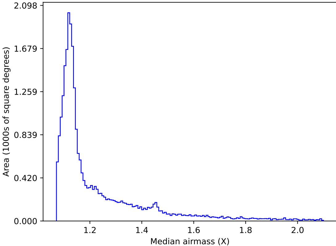
noroll_mjdp365_v3.4_10yrs All sky r band: Median airmass
