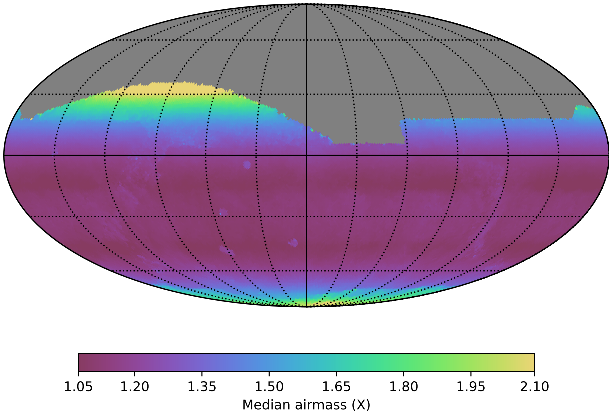
noroll_mjdp365_v3.4_10yrs All sky i band: Median airmass
