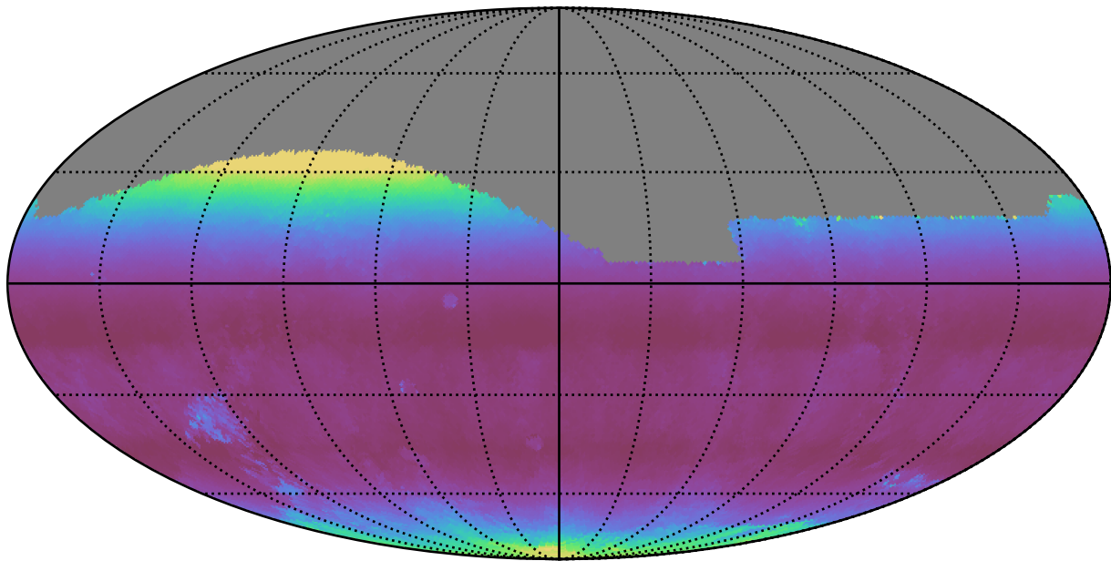
noroll_mjdp365_v3.4_10yrs All sky g band: Median airmass
