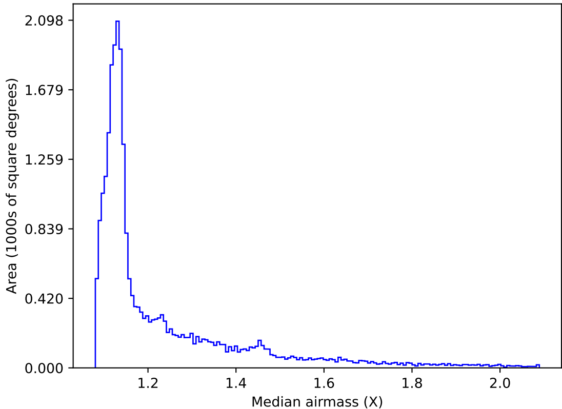
noroll_mjdp365_v3.4_10yrs All sky all bands: Median airmass
