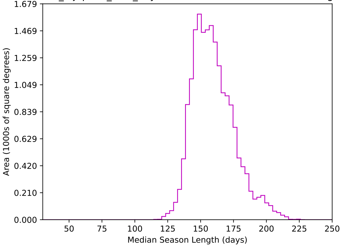
noroll_mjdp365_v3.4_10yrs WFD z band: Median Season Length
