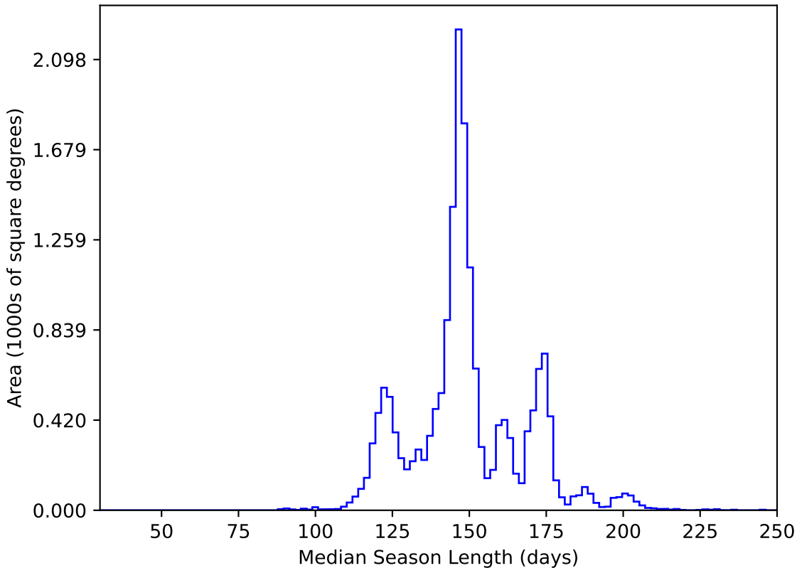
noroll_mjdp365_v3.4_10yrs WFD y band: Median Season Length
